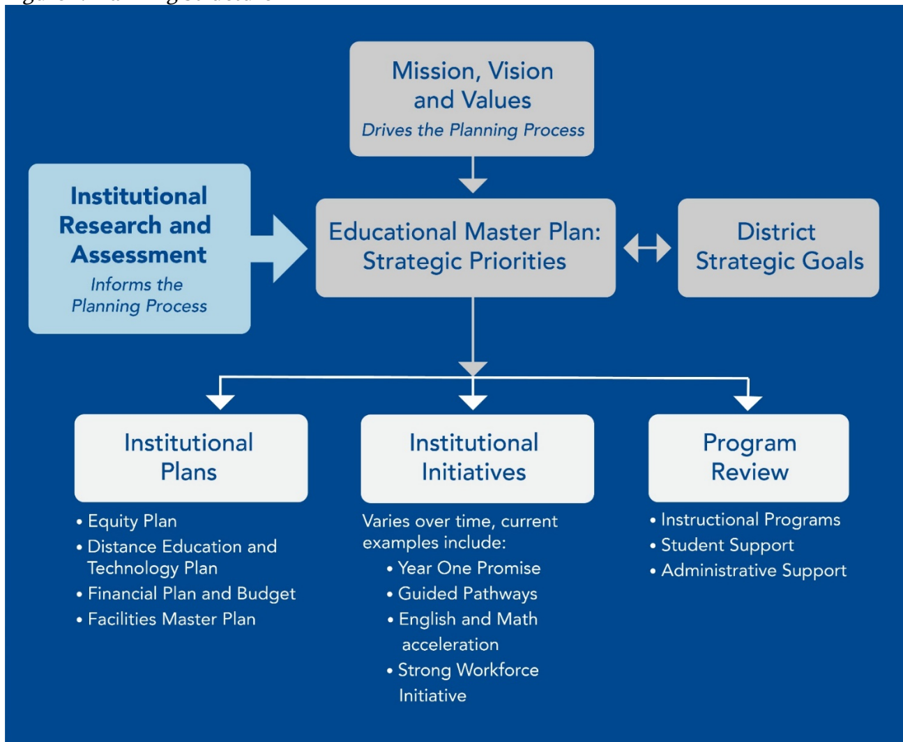
Figure 1: Planning Structure
